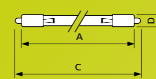
Single Pin
